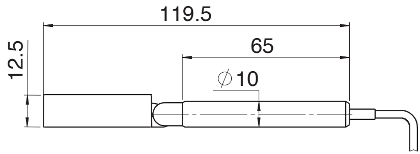
VIEW A
