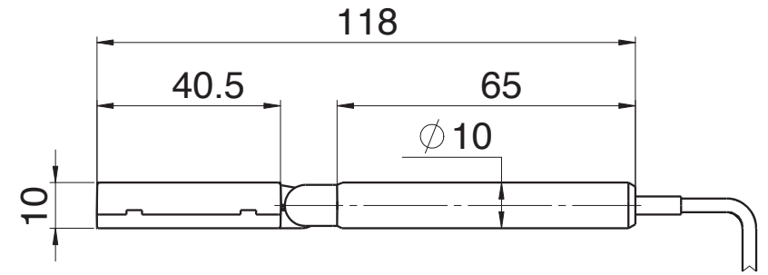
VIEW A
